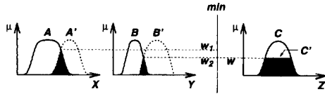
Fig. 9. Approximate reasoning for multiple antecedents.
