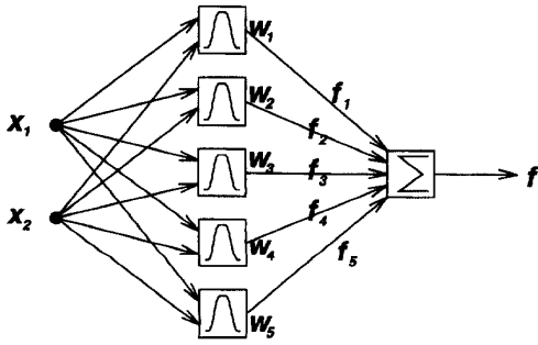
Fig. 27. A radial basis function network (RBFN).
