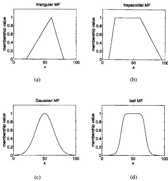
Fig. 3. Examples of various classes of MF's: (a) triangle ( x ; 20, 60, 80); (b) trapezoid ( x ; 10, 20, 60, 95); (c) gaussian ( x ; 20, 50); (d) bell ( x ; 20, 4, 50).
